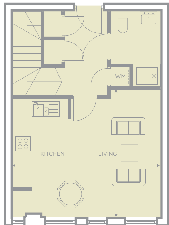
GROUND
